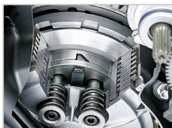
Adjustable back-torque limiting clutch
